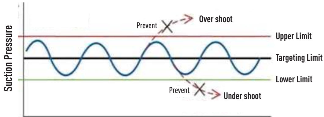
Suction Pressure Fluctuation of Normal machine
